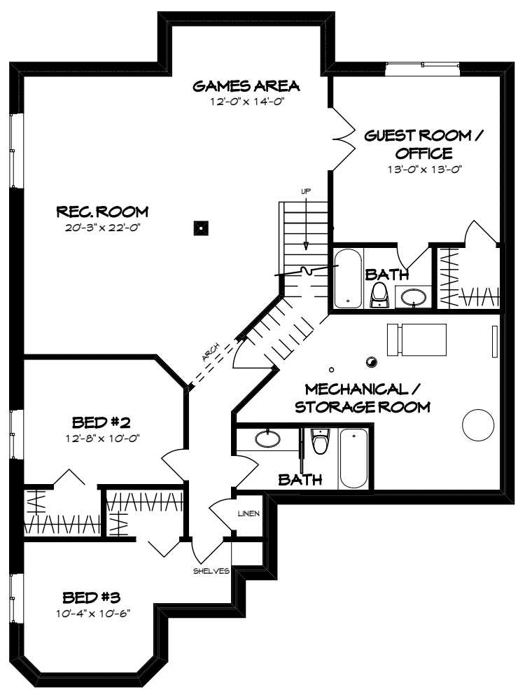
LOWER FLOOR PLAN 1925 FEET SQ.
